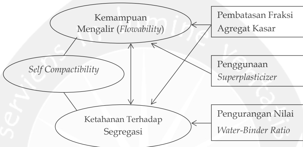
Gambar 2.1 Prinsip Dasar Proses Produksi Self-Compacting Concrete (Dehn dkk, 2000)
