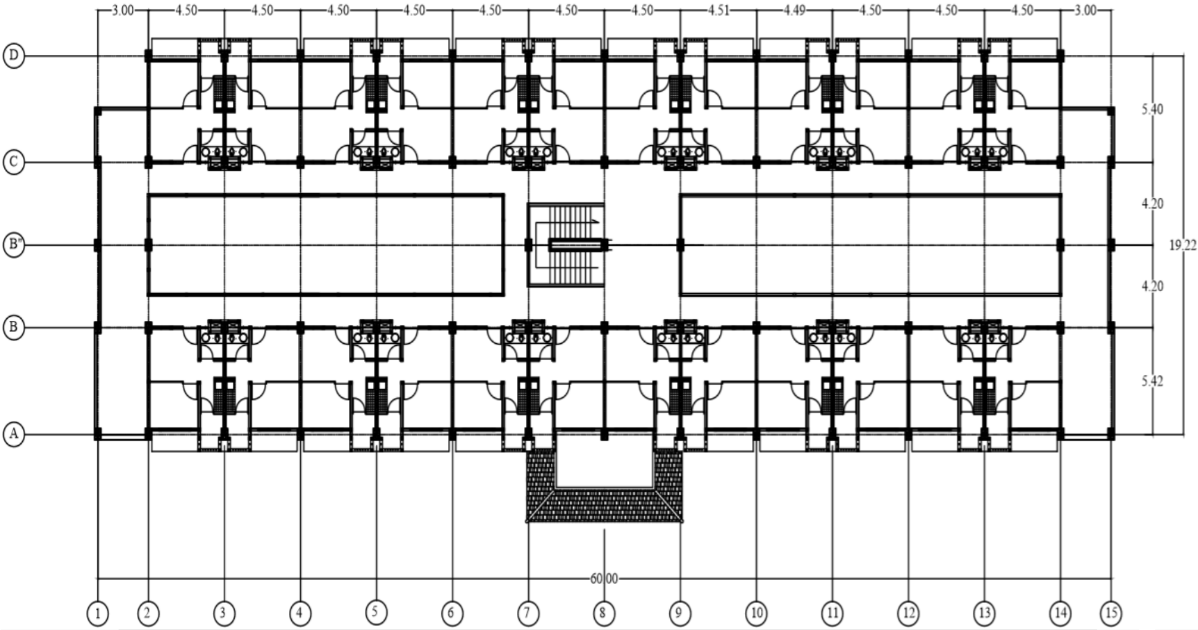
Denah Lantai lantai 1
