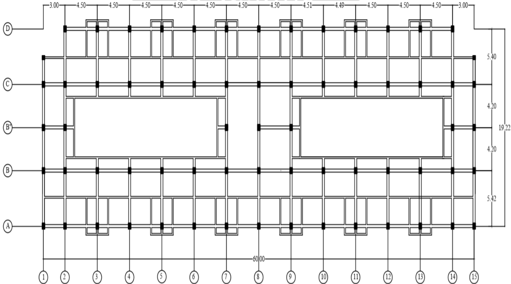
Denah Balok Lantai 2-6
