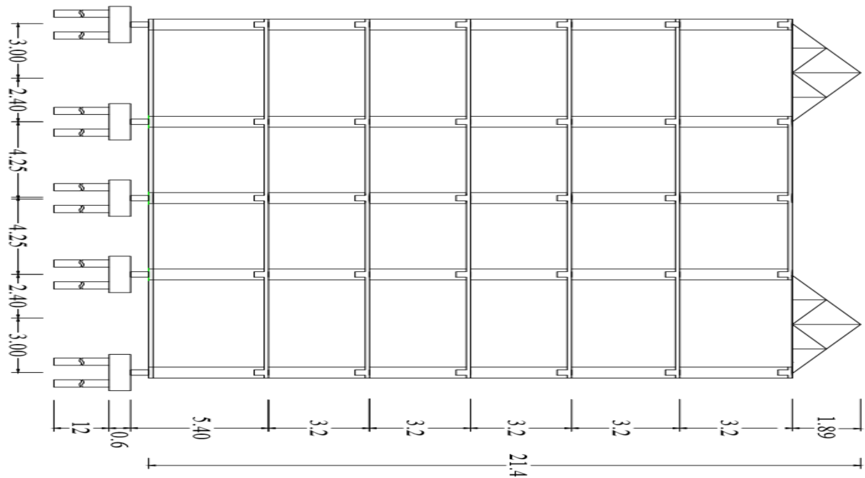
GAMBAR PORTAL
