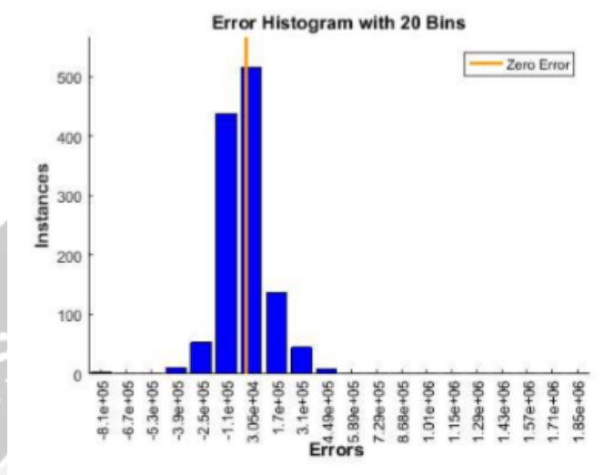
Gambar 7 Error histogram
