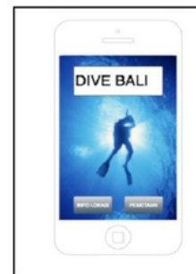
Fig. 5. Main Page
