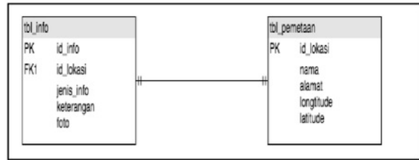
Fig. 4. Database Conceptual
