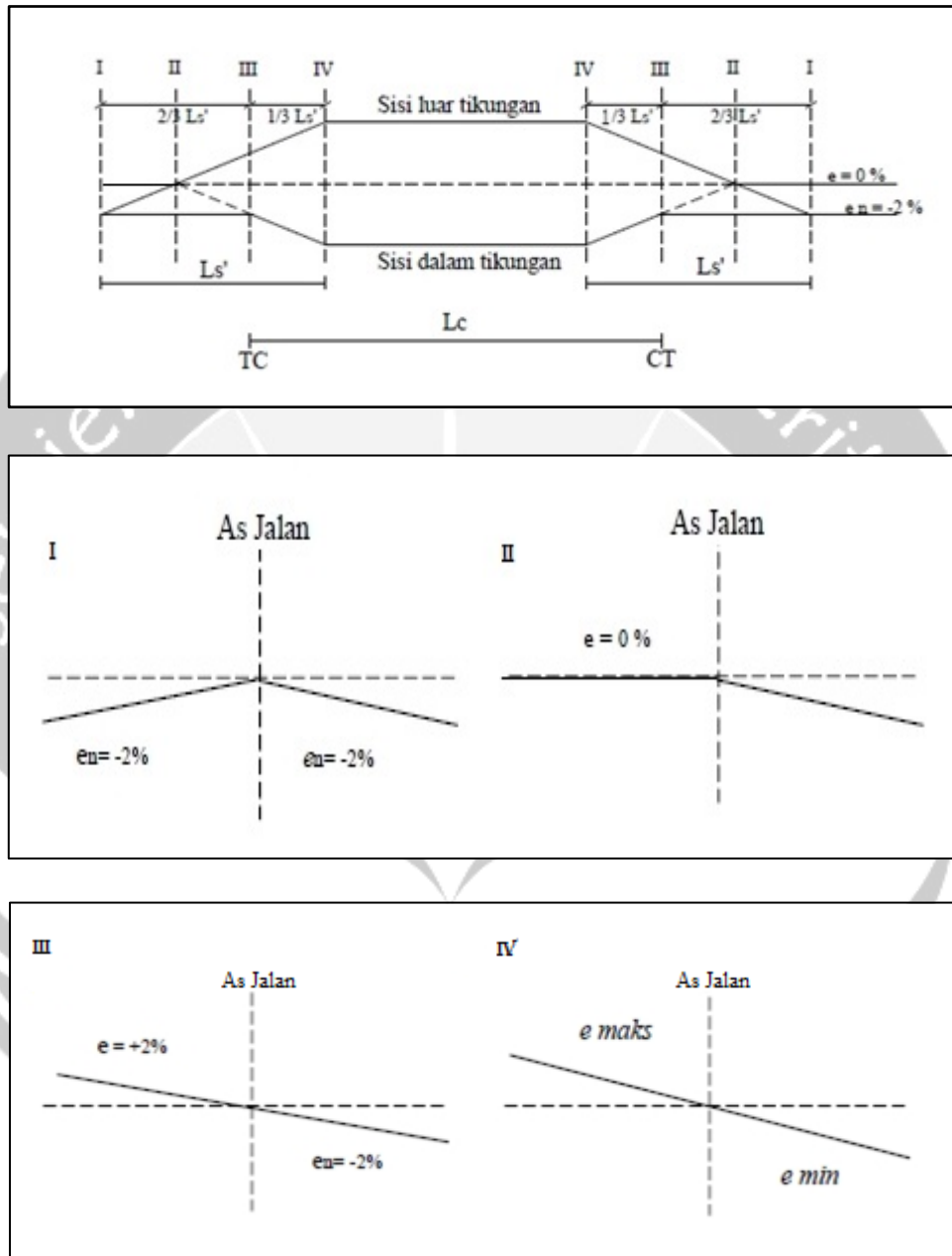
Gambar 3.10 Diagram Superelevasi Full Circle
