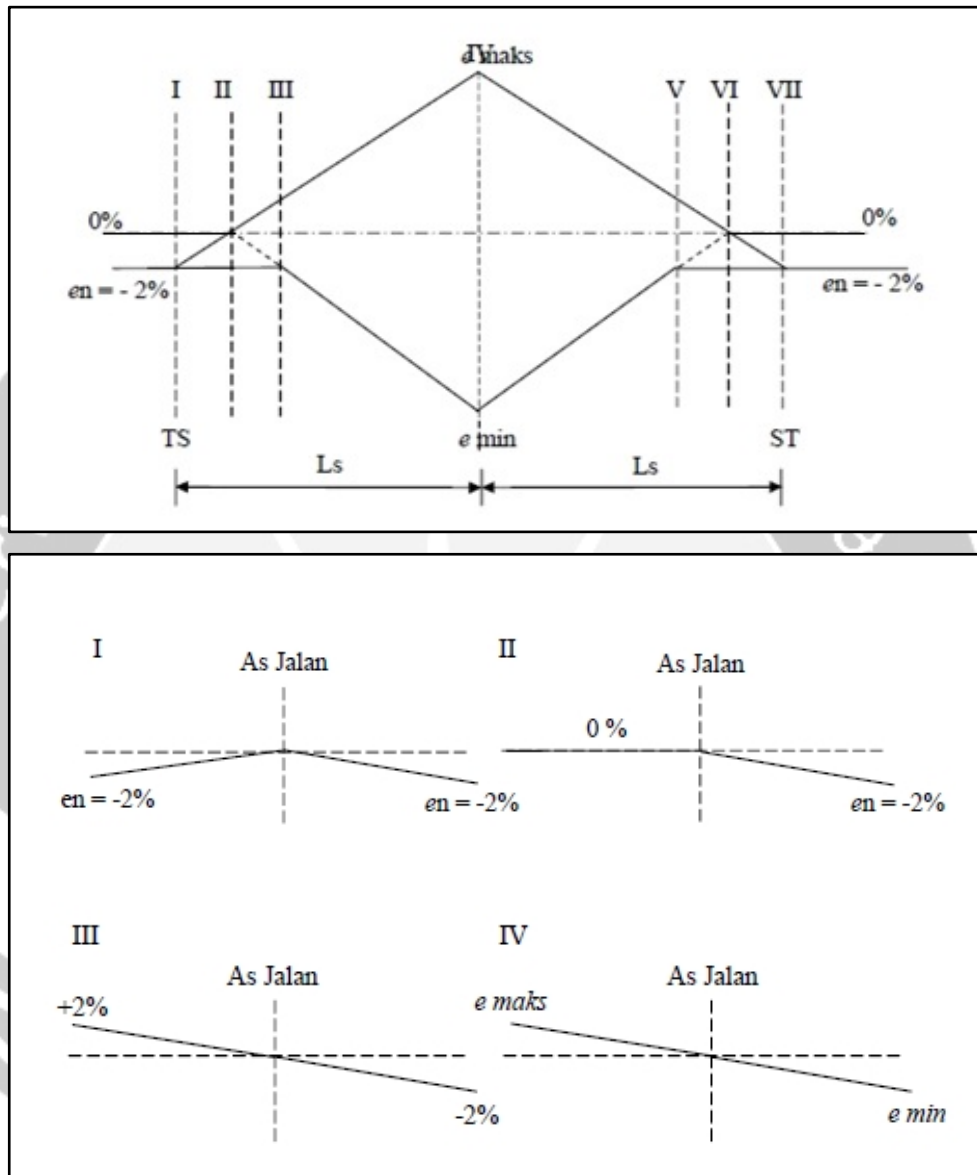
Gambar 3.12 Diagram Superelevasi Spiral-Spiral Sumber : Hendarsin (2000)
