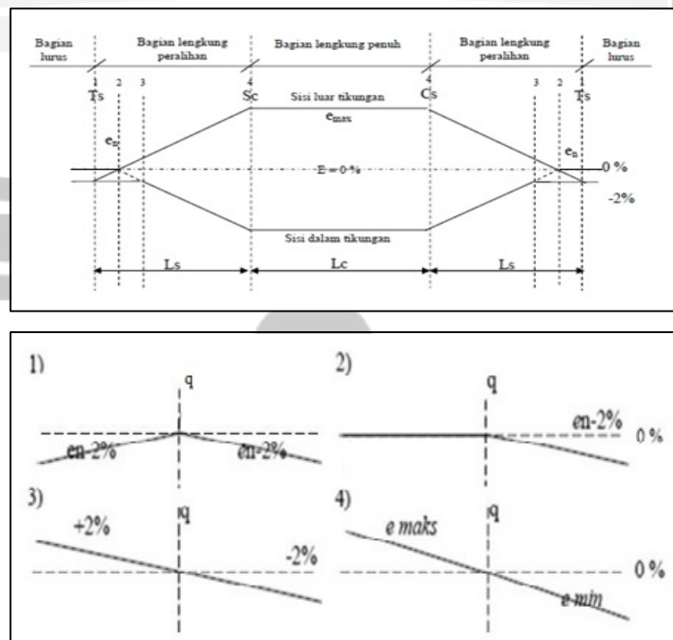
Gambar 3.11 Diagram Superelevasi Spiral-Circle-Spiral
