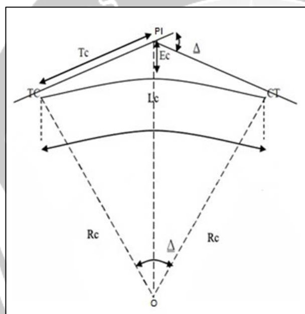
Gambar 3.6 Lengkung Full Circle
