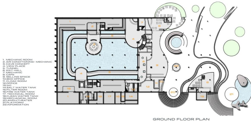
Gambar 2.26 Ground Floor Antalya Aquarium Sumber : www.archdaily.com
