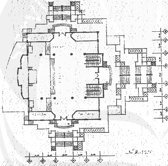
Denah lantai 2
