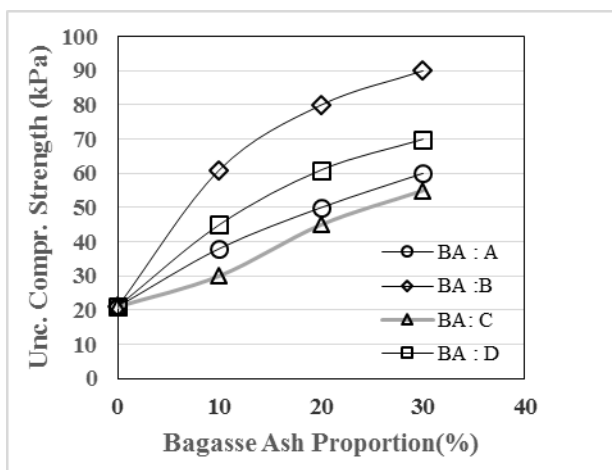
Fig. 3. Unconfined Compression Strength of Soil Z
