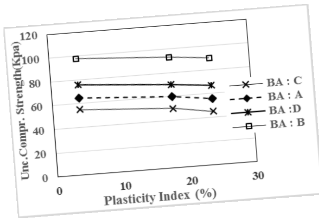
Fig. 8. Relations between Unc. Compr. Strength and Plasticity Index
