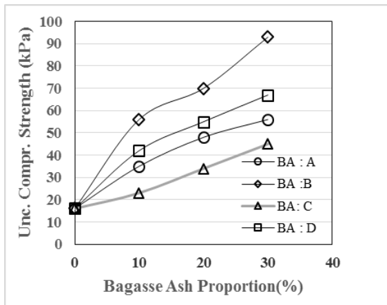
Fig. 1. Unconfined Compression Strength of Soil X
