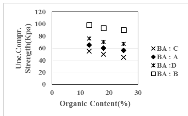
Fig. 7. Relations between Unc. Cmpr. Strength and Organic Content
