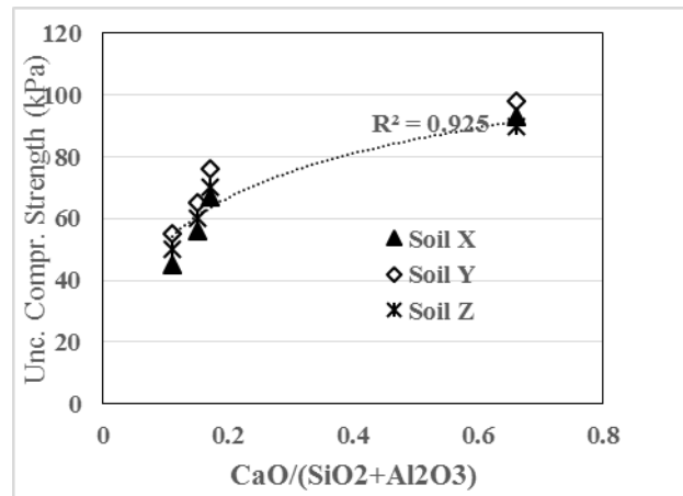
Fig. 6. Relations between Unc. Cmpr. Strength and CaO/(SiO 2 +Al 2 O 3 )
