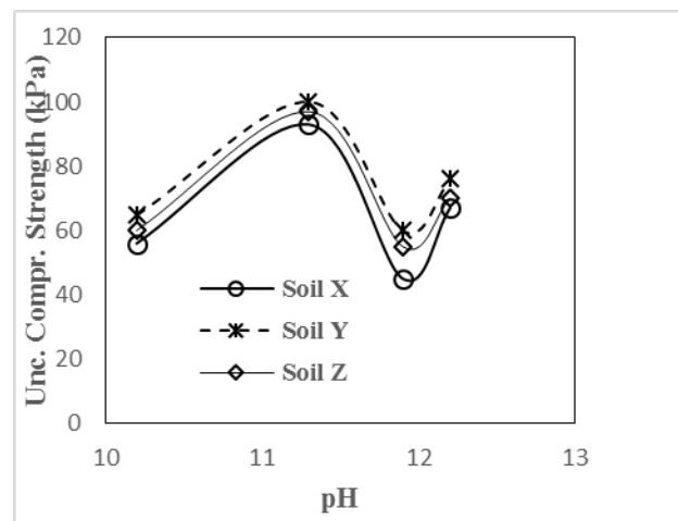
Fig. 4. Relations between Unc. Cmpr. Strength and pH
