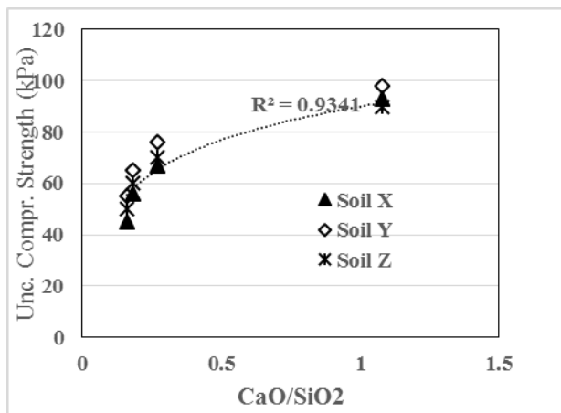
Fig. 5. Relations between Unc. Cmpr. Strength and CaO/SiO 2
