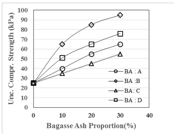
Fig. 2. Unconfined Compression Strength of Soil Y
