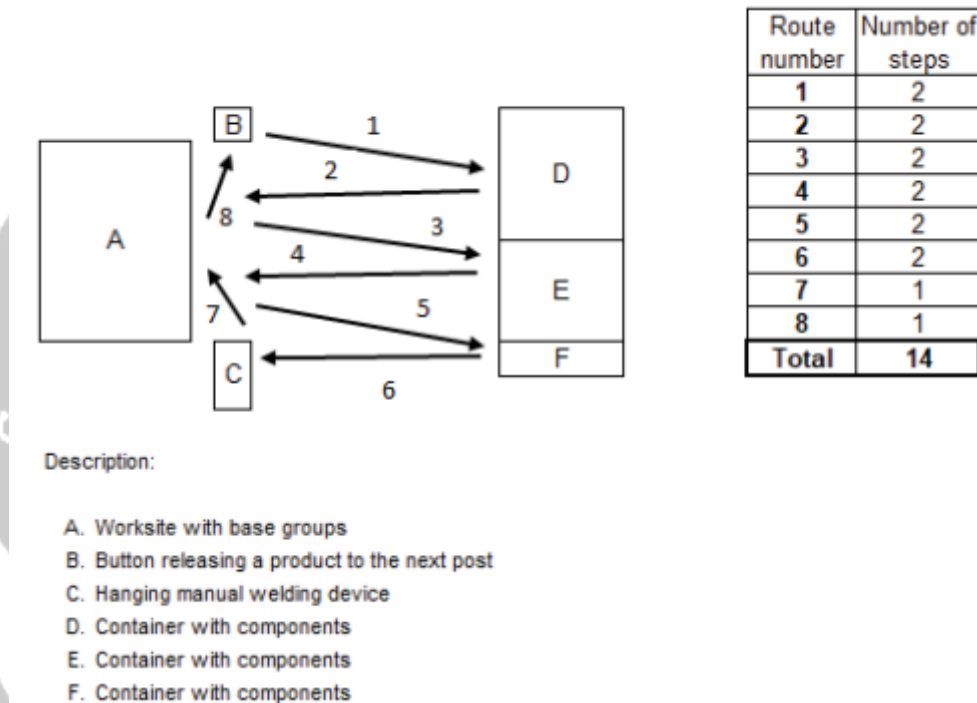
Figure 2. 2. Spaghetti Diagram Example (Domagala, 2018)
