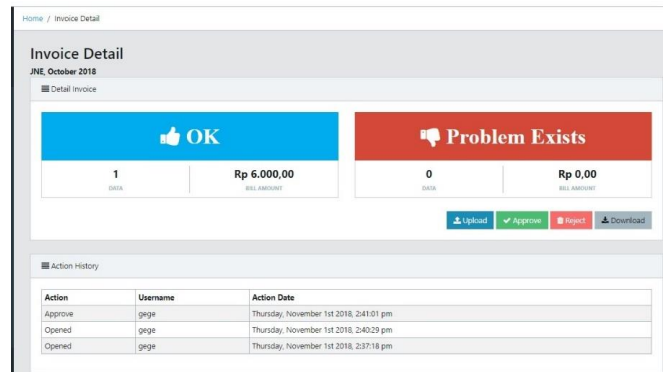
Fig 9. Validation Dashboard
