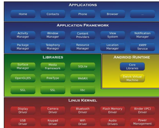
Figure 1. Android System Architecture (Gu et al., 2014)
