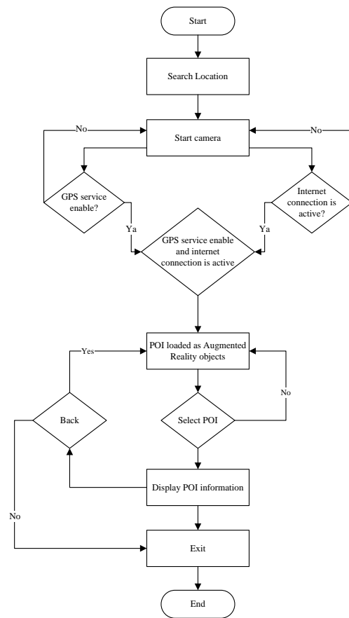
Figure 4. System Flowchart
