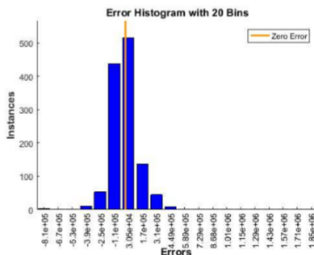
Gambar 7 Error histogram
