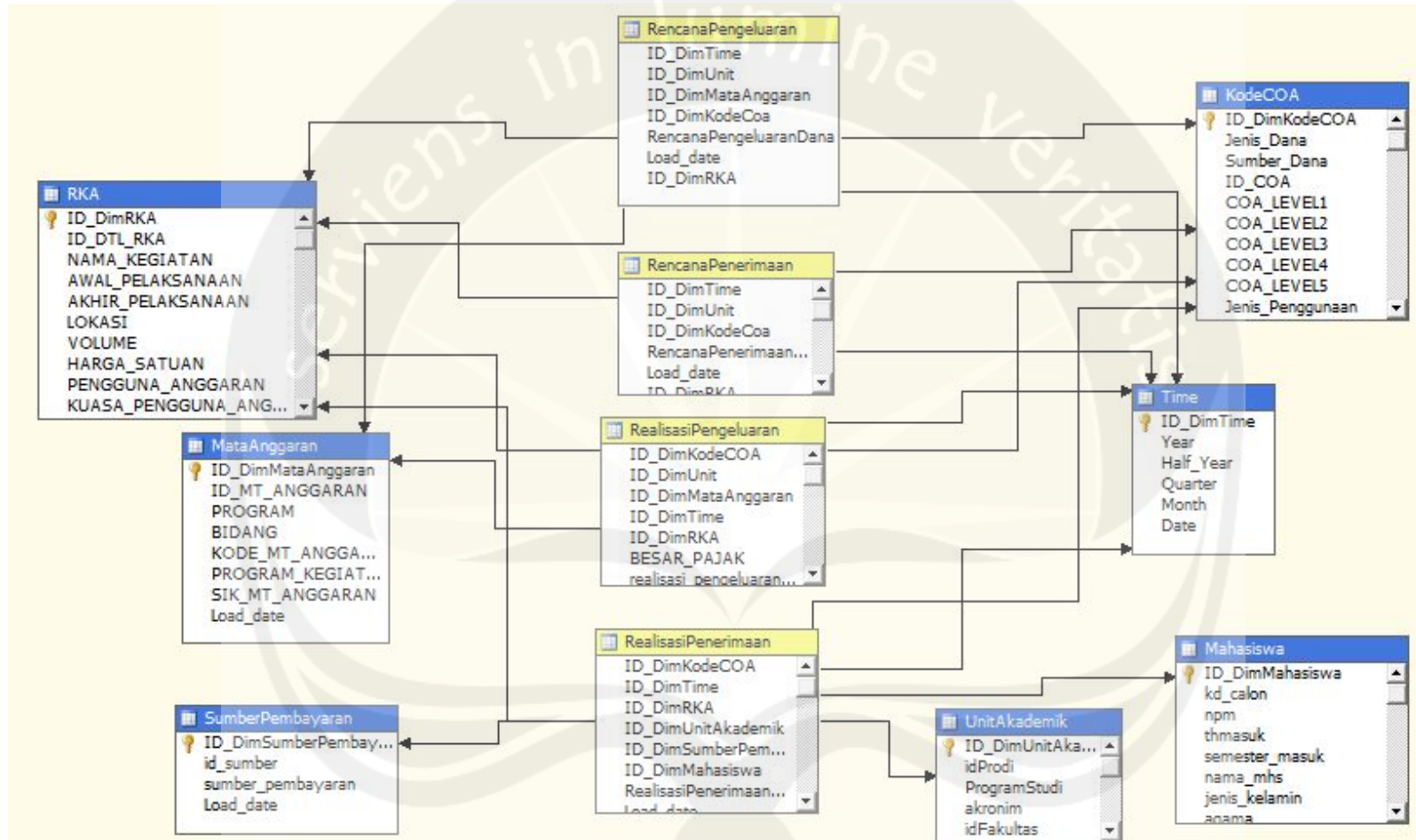
Gambar 3.1. Physical Data Model
