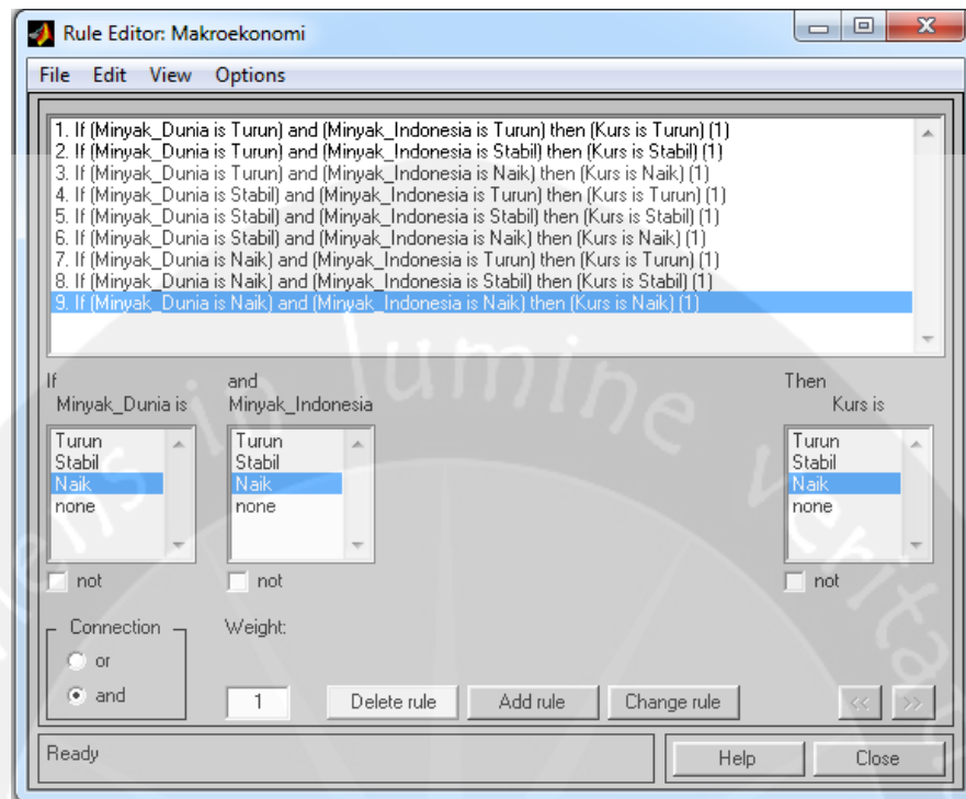
Lampiran 1.39 Rule Kurs
