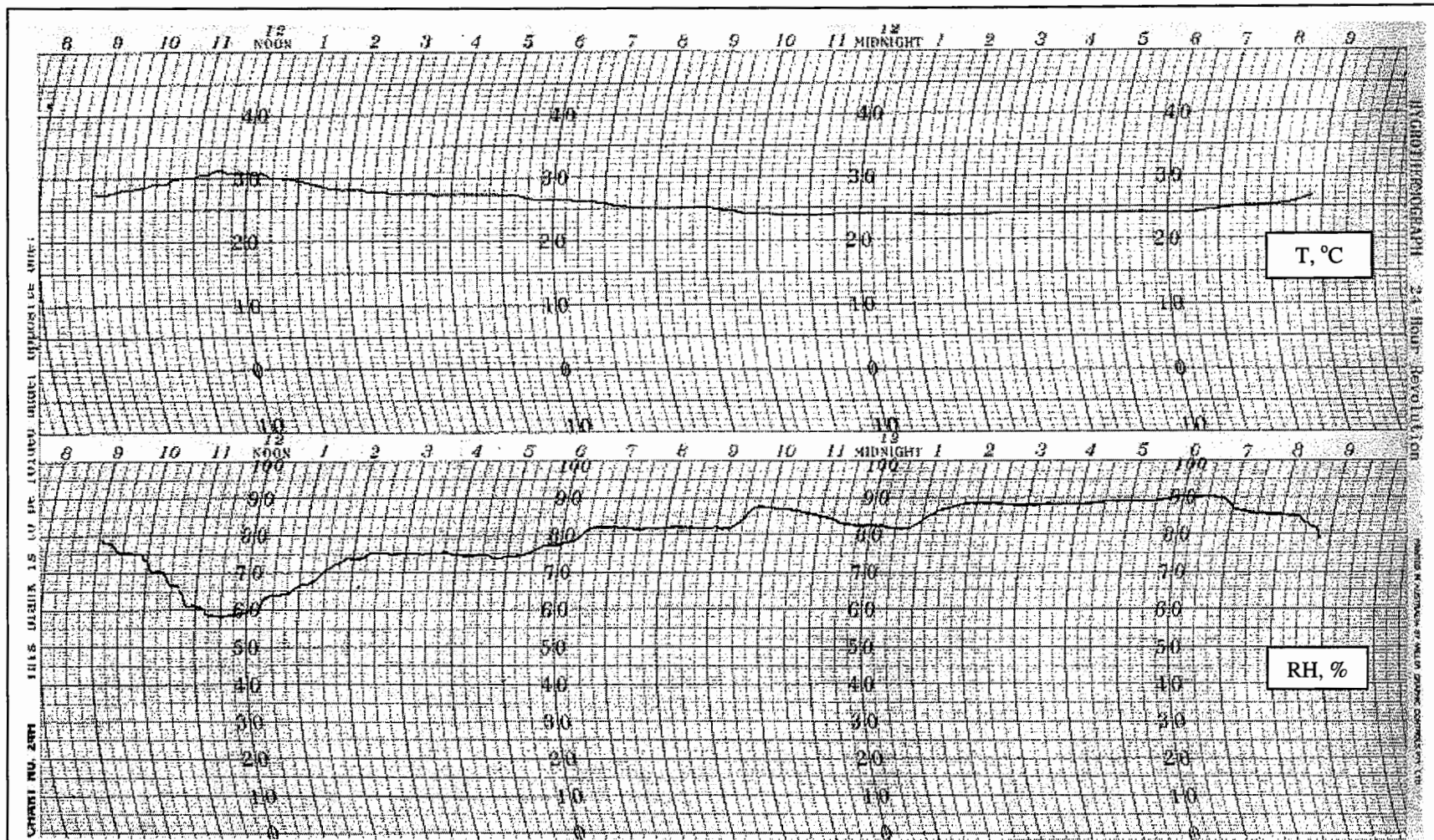
Figure 3-13 Twenty-four hours' recording of air temperature and humidity in a clear day, 6 November 1996. The highest air temperature, 31°C, was reached around 12:00. The lowest air temperatures, 24°C were between 21:00 and 06:00. The low relative humidity, 59%, high humidity, 90%, were found around 12:00 and 06:00 respectively. Location: Demangan, Yogyakarta.
