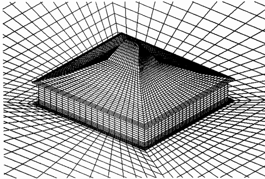
Figure 9-13 The grid design of a Joglo kitri model based on structured grid system (generated using CFD-GEOM).
