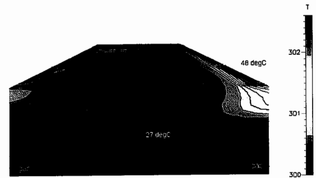
Joglo kitri (S) with gaps above floor
