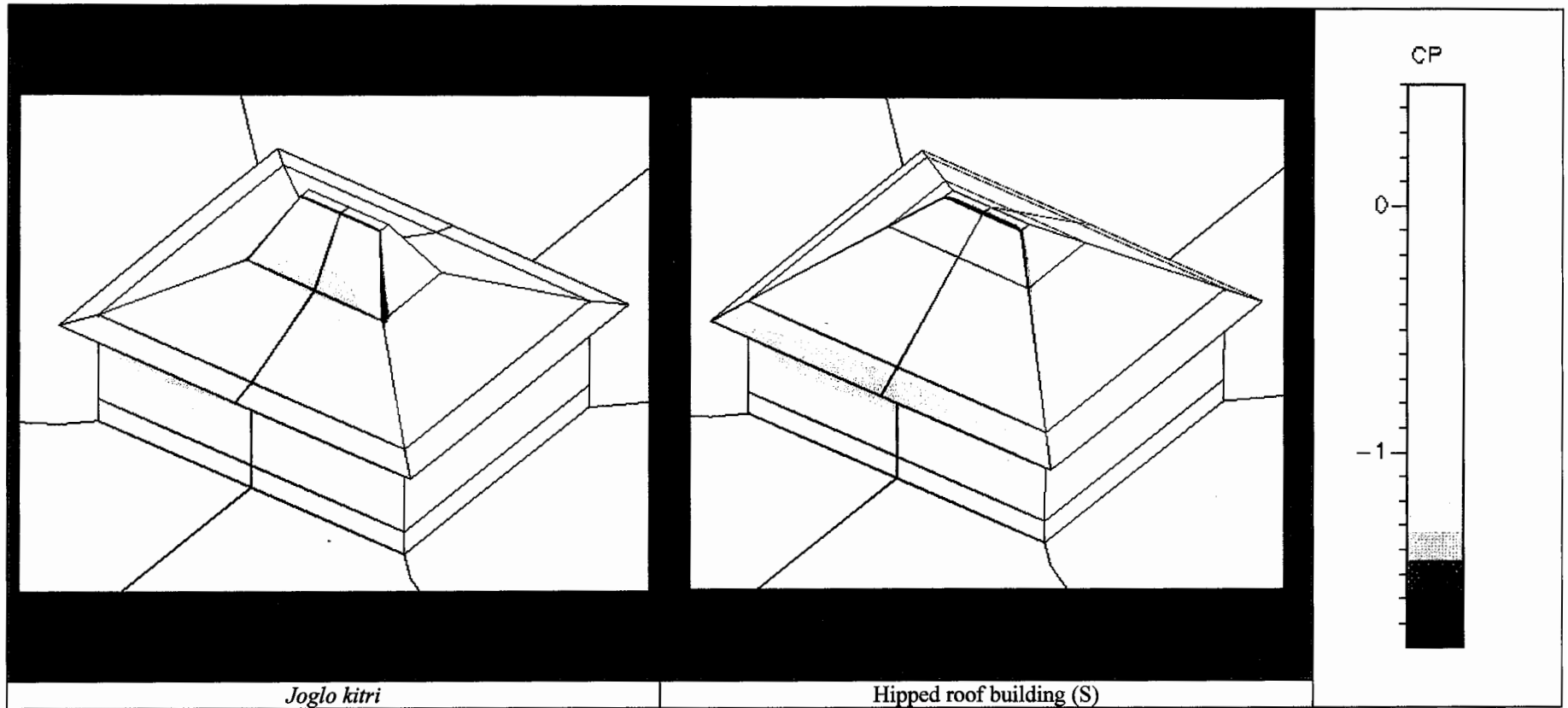
Figure 11-2 Comparison of pressure coefficient ( C_p ) distribution at roof surfaces of Joglo kitri (S) and the hipped roof building (S). Folded line between guru and pananggap sectors creates high positive pressure area. The ventilation potential at roof level of Joglo kitri is higher than that of the hipped roof building.
