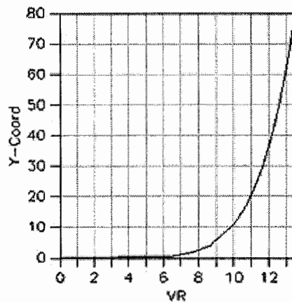
Figure 8-3 Atmospheric boundary layer wind profile
