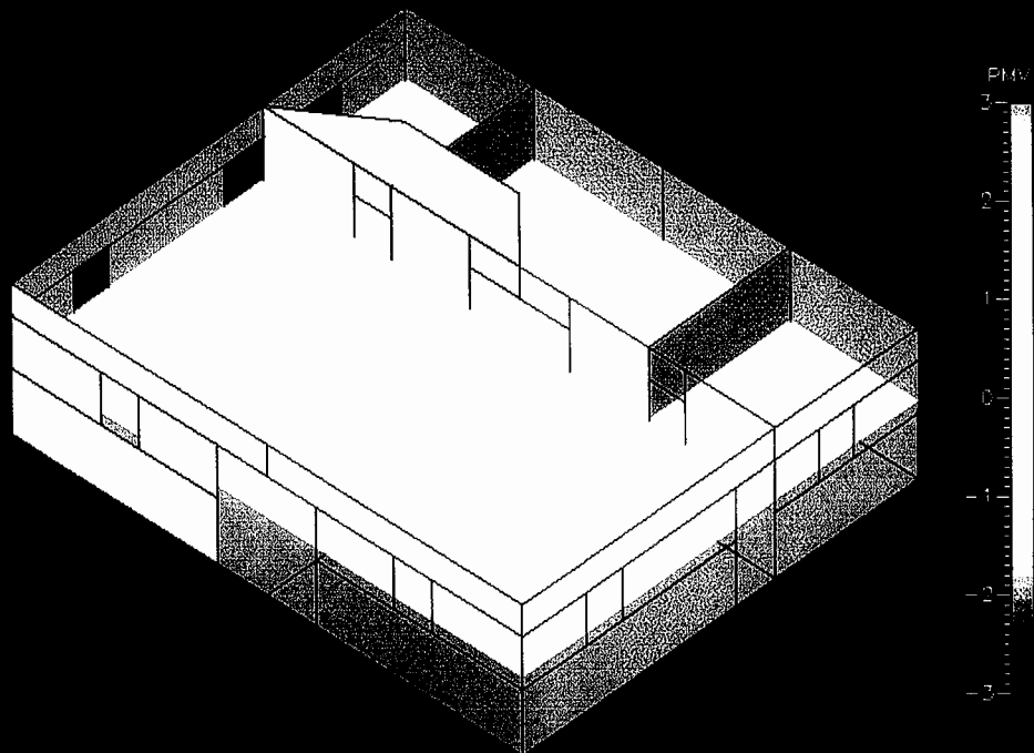
Figure 10-17 Predicted Mean Vote inside Joglo sri for a person doing sedentary work, wearing trousers and a long sleeve shirt. Senthong kiwa and Senthong tengen are slightly too warm. Other places are comfortable.
