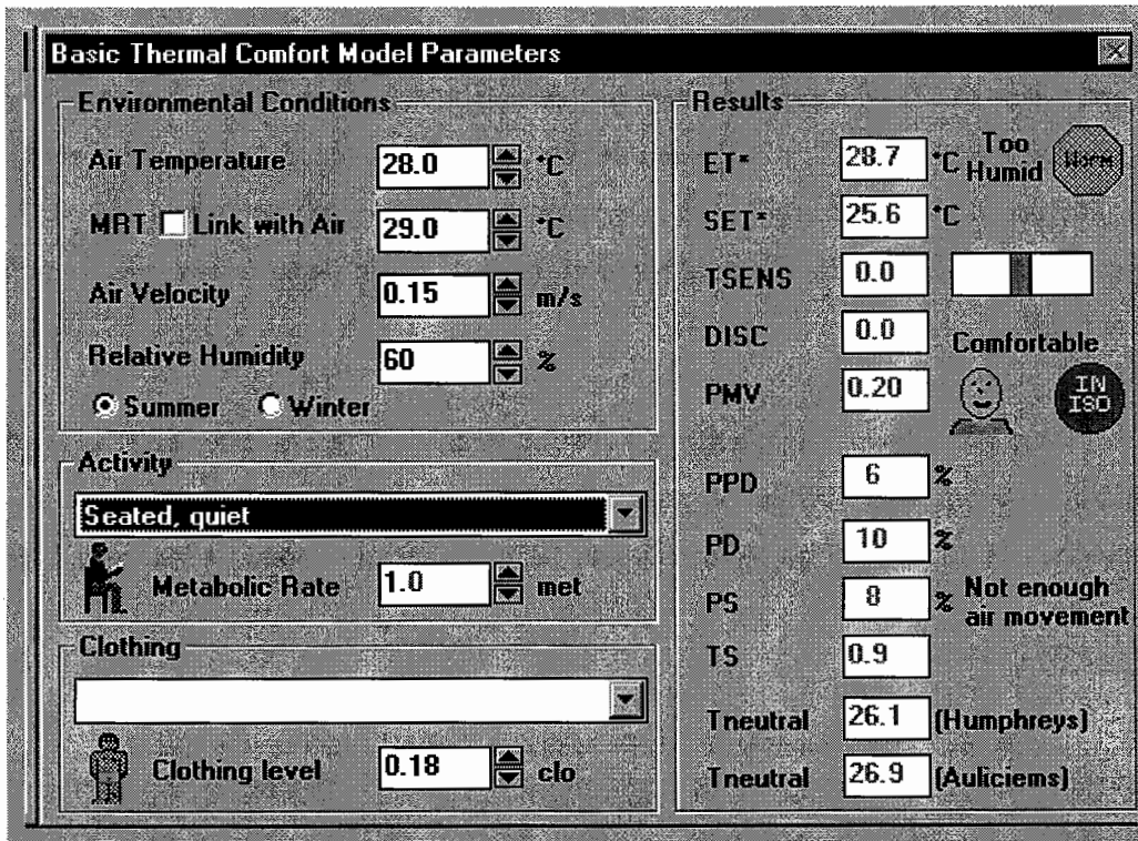
Figure A-1 An example of a simple evaluation to the data presented at Table A-3.
