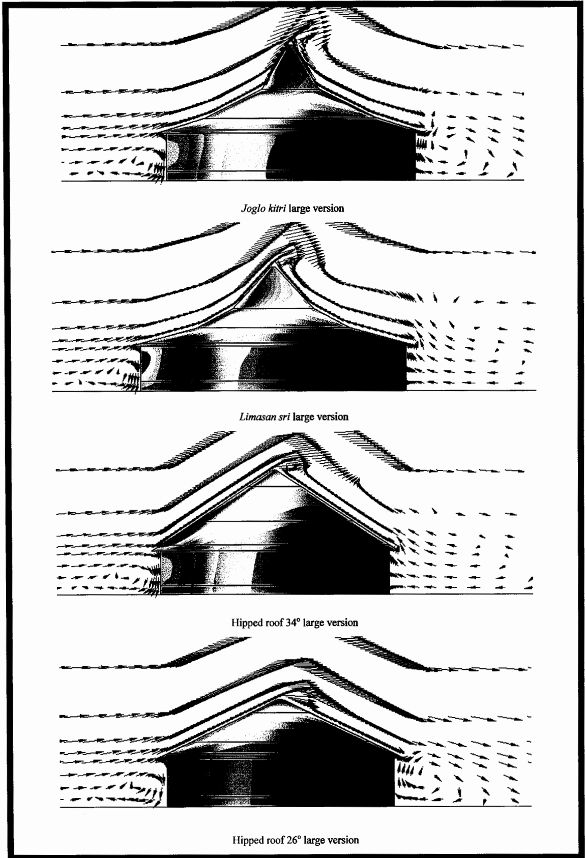
Figure 9-27 Vectors around large version models.
