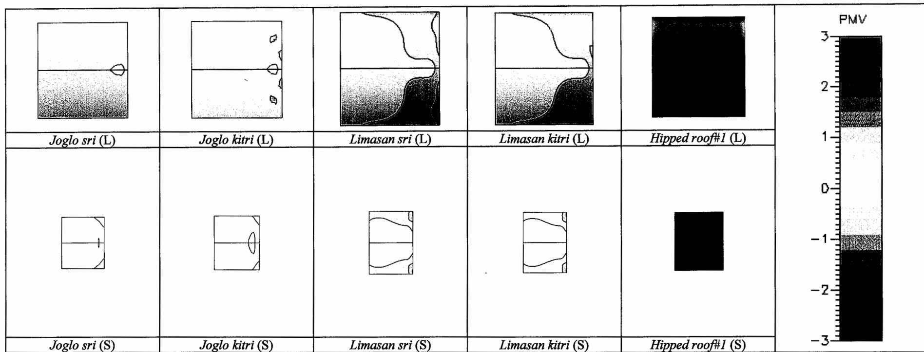
Figure 10-8 Comparison of Predicted Mean Votes (PMV) distribution at 120 cm above the floor. Senthong tengah (northern part) is the most thermally comfortable place. Small Javanese buildings are more comfortable than the large ones. Non-Javanese (hipped roof) buildings are thermally uncomfortable.
