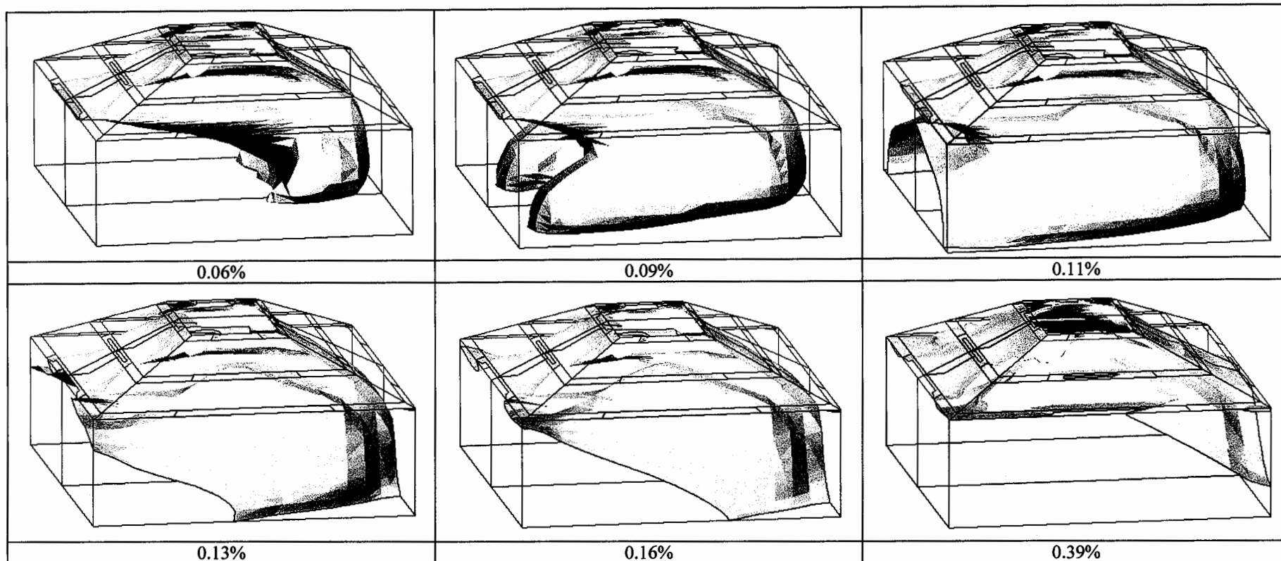
Figure 10-9 Area of various Predicted Percentage of Dissatisfied (PPD) in Joglo sri under an average climate condition (scenario Table 10-6). The occupants' zone is thermally comfortable. PPD = 0.39% means less than one person of a hundred will complain about the indoor climate. Location of senhong tengah is the most comfortable.
