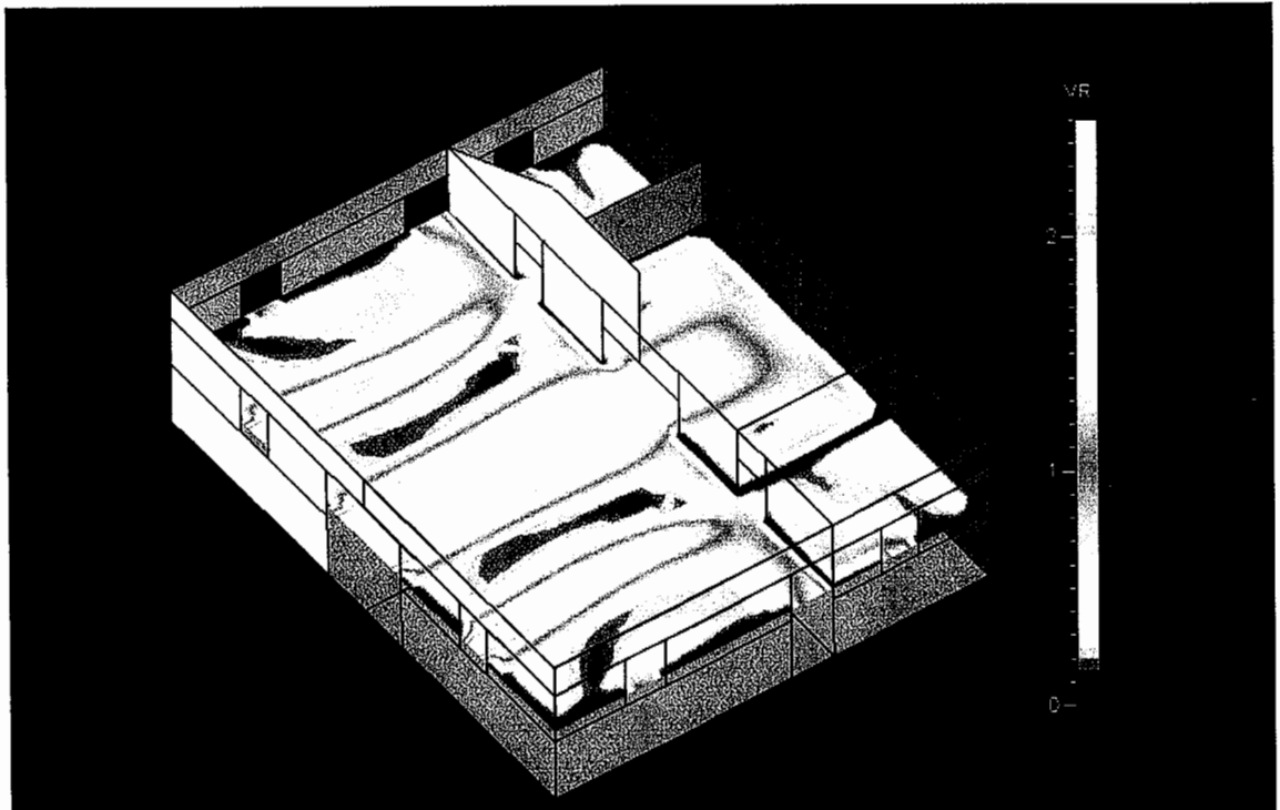
Figure 10-14 Air velocity distribution inside Joglo sri , 120 cm above the floor. Air velocities in Senthong kiwa and Senthong tengen are lower than those in Senthong tengah .
