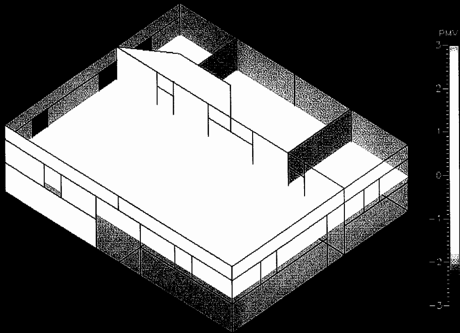
Figure 10-16 Predicted Mean Vote inside Joglo sri for a person wearing short and T-shirt. Senthong kiwa and Senthong tengen are thermally comfortable. Other places are slightly cool.
