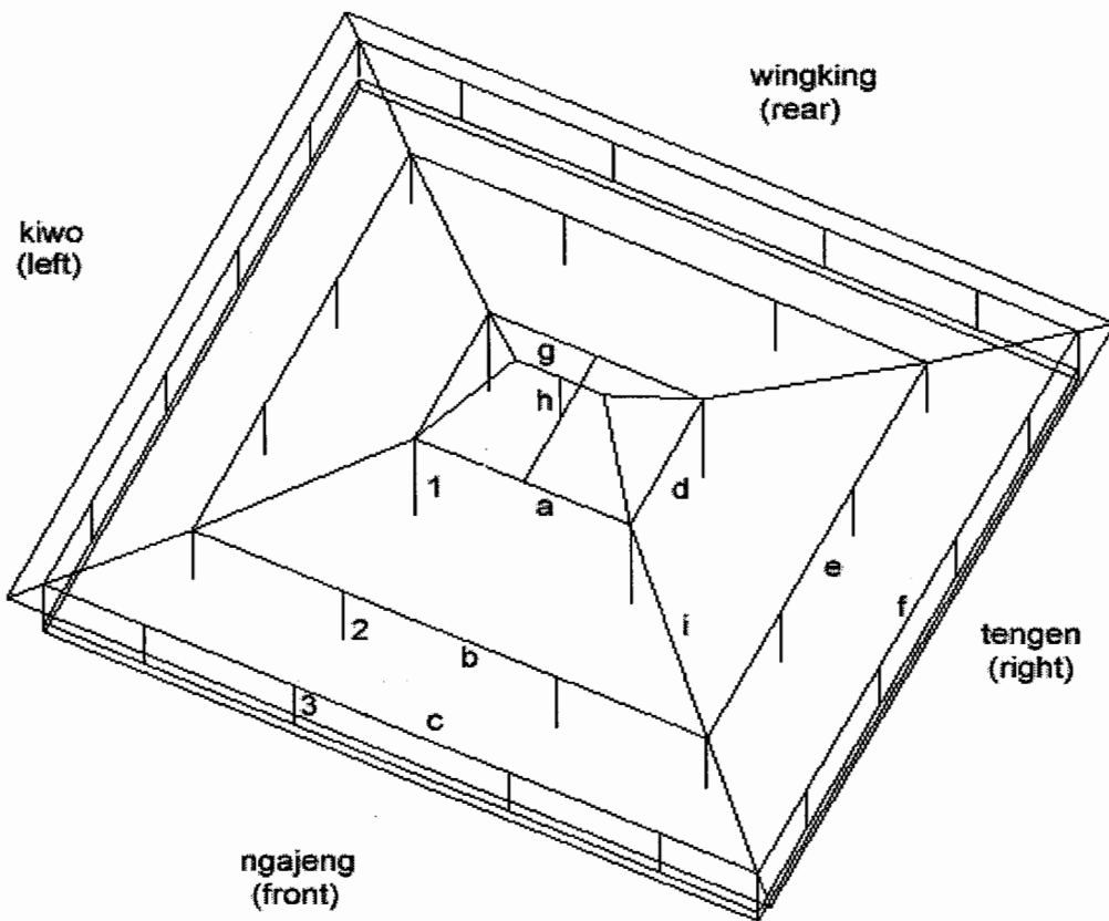
Figure 4-4 Parts of Javanese building structure
