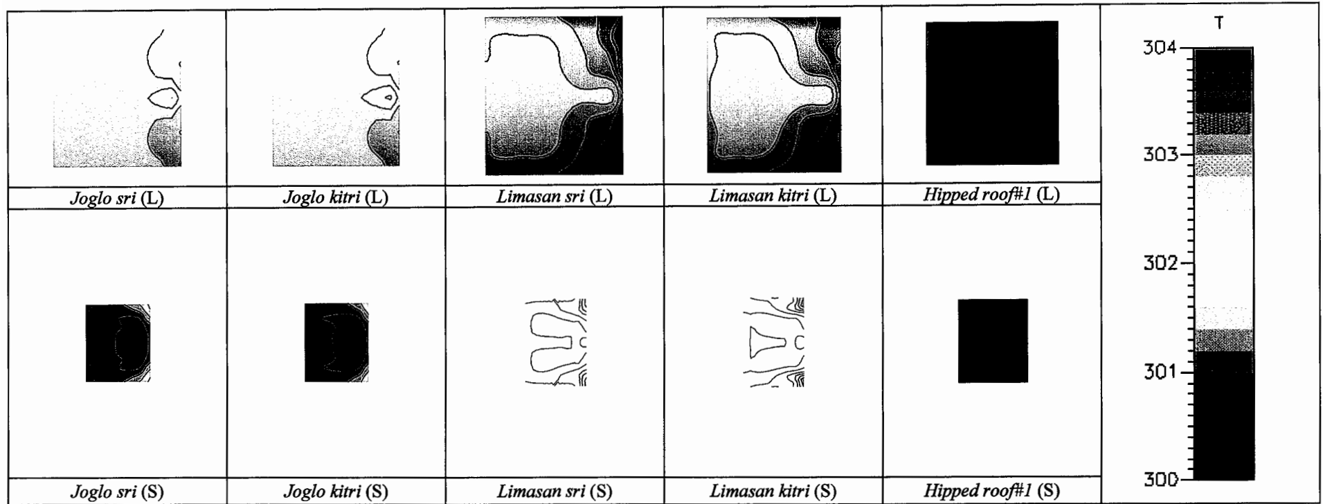
Figure 10-7 Comparison of air temperature distribution at 120 cm above the floor. Senthong kiwa (upper right hand side) and senthong tengen (lower right hand side) are warmer than other parts of the buildings. Senthong tengah (middle right hand side) is cooler than other parts of the building. Hipped roof buildings are evenly hot.
