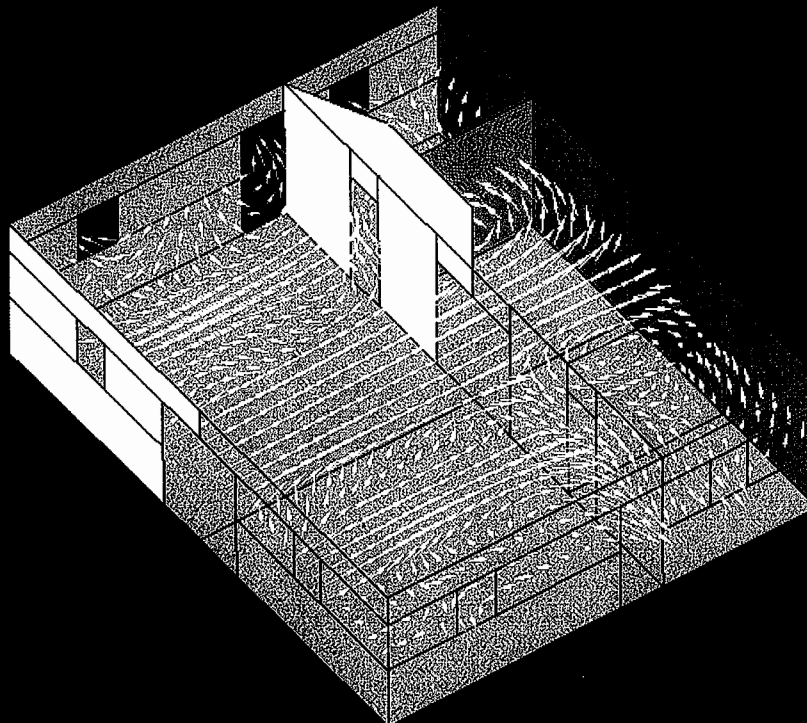
Figure 10-19 Airstream inside Joglo sri , at 120 cm above the floor. Vectors show the air path from the south wall's openings to the east and west walls' openings.
