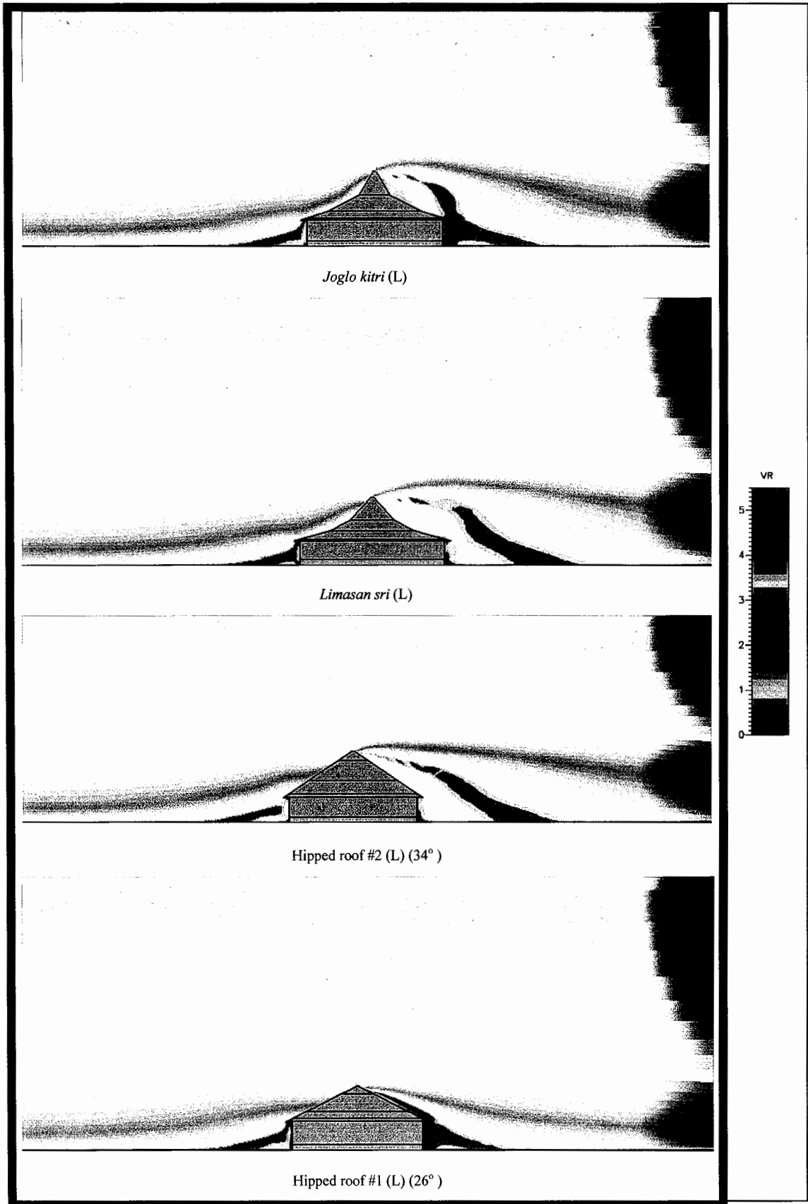
Figure 9-25 Comparison of air velocity distribution around large version models.
