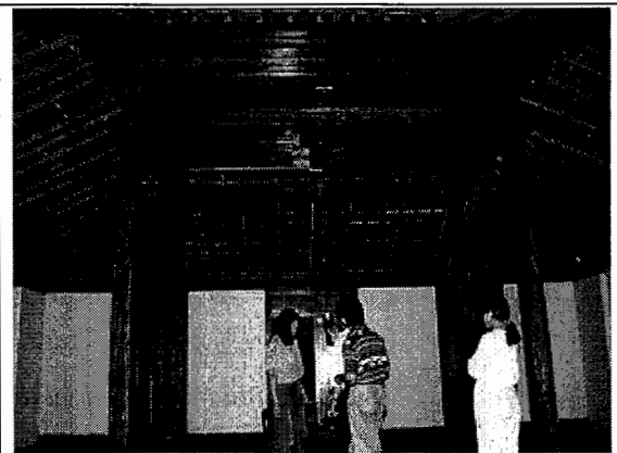
Figure 5-4 Redundant construction of tumpang sari . Its actual strength is 300 to 700% higher than it needs to be.
