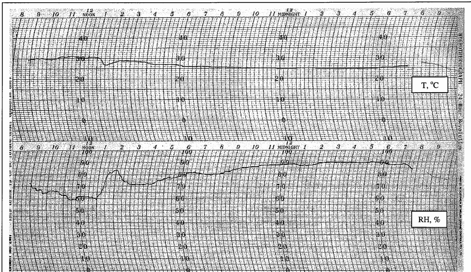
Figure 3-12 Twenty-four hours' recording of air temperature and humidity on 5 November 1996 with a short period of rain. The highest air temperature, 31°C, is between 11:00 and 13:00. The low air temperature, 25°C, is between 21:00 and 06:00. A short rainfall caused a short fall of air temperature between 13:00 and 14:00. On the other hand, between 11:00 and 13:00 the relative humidity was low and between 21:00 and 06:00 it was high. The lowest relative humidity of 59% was at 11:30. The highest relative humidity of 90% was from 03:00 to 06:00. Location: Demangan, Yogyakarta.
